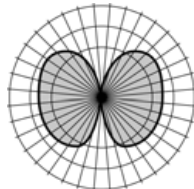
Elevation radiation pattern
