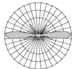
Elevation radiation pattern
