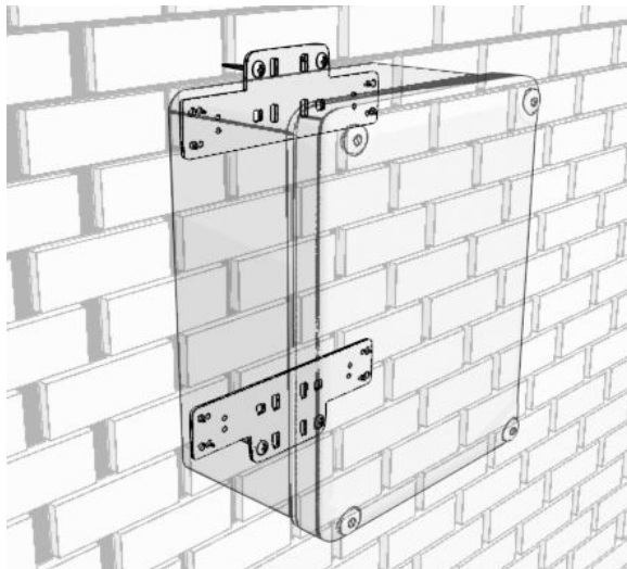
The UMB used in a wall mounting set up
