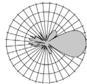
Elevation radiation
